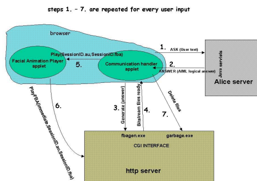
Figure 2: System architecture of the "Intelligent" Virtual Talking Character Demy
